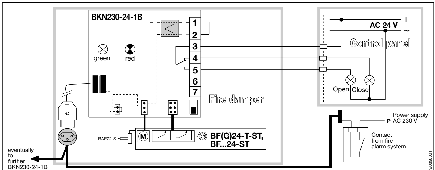
Typical wiring diagram BKN 230-24-1B without BKS24-1B
