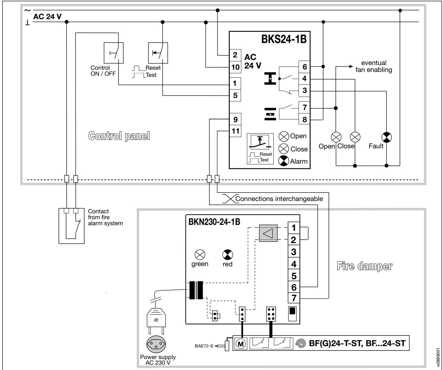
Typical wiring diagram BKN230-24-1B with BKS24-1B
