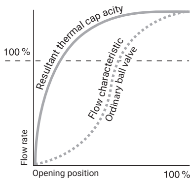
Characteristic of an ordinary ball valve
